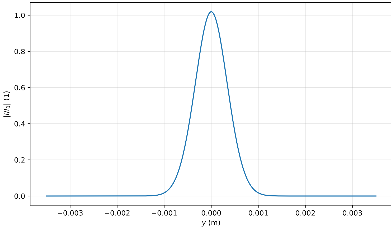
Intensity profile I(x=0, y, z=0.239)/I_0 , P_{in}=0.6P_{cr} , artificial time
